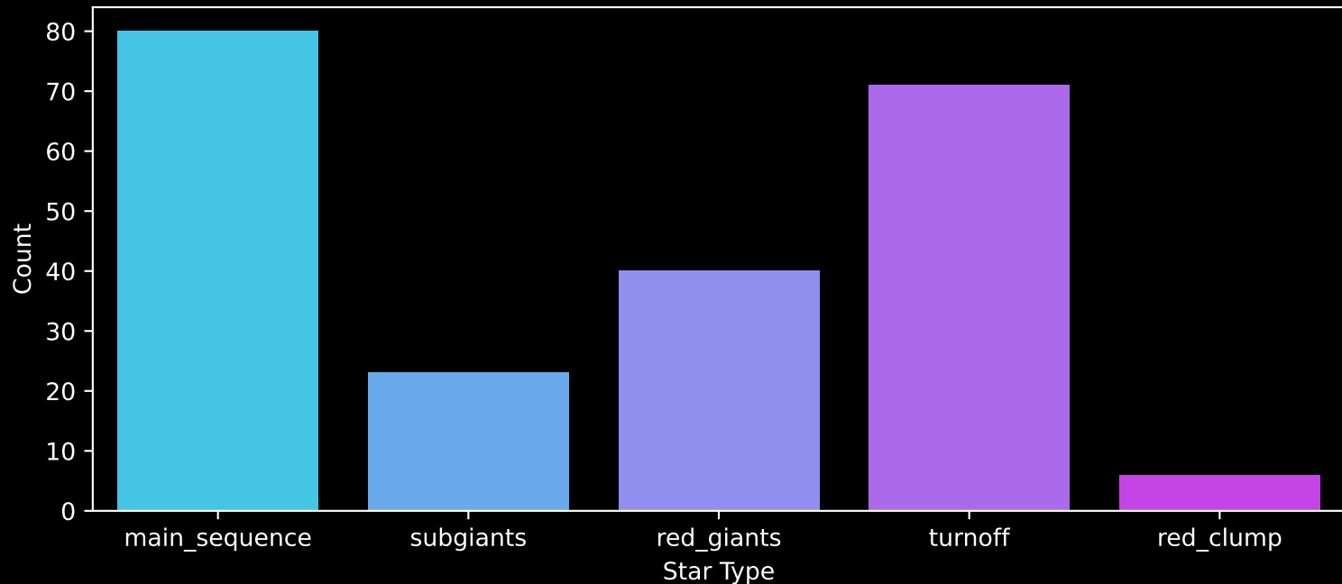
GALAH DR4 Field: [7151] Count plot of Star Type
