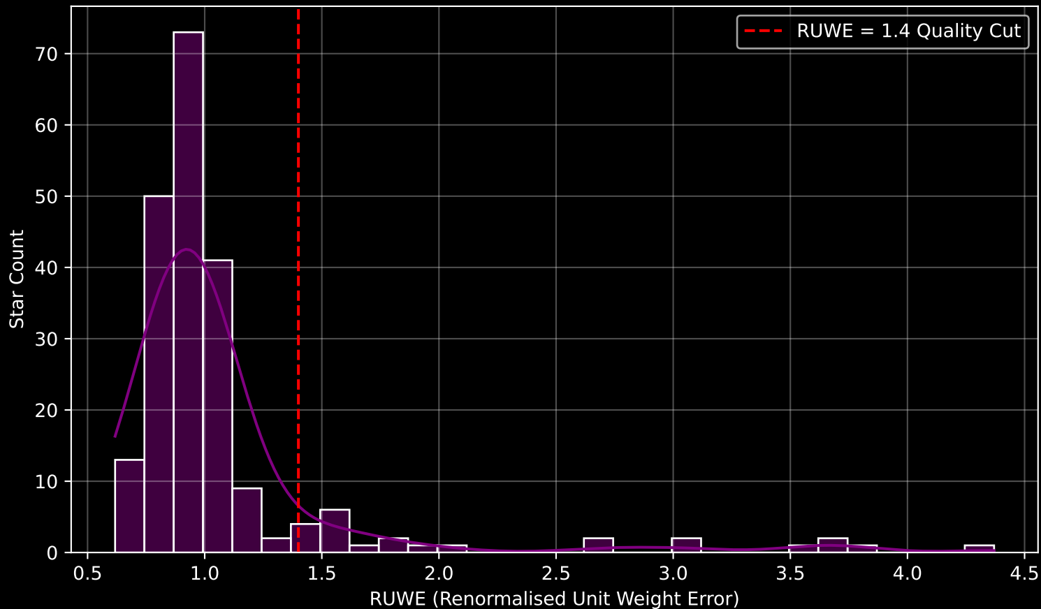
GALAH DR4 Field [7151] RUWE Distribution (n= 212)
