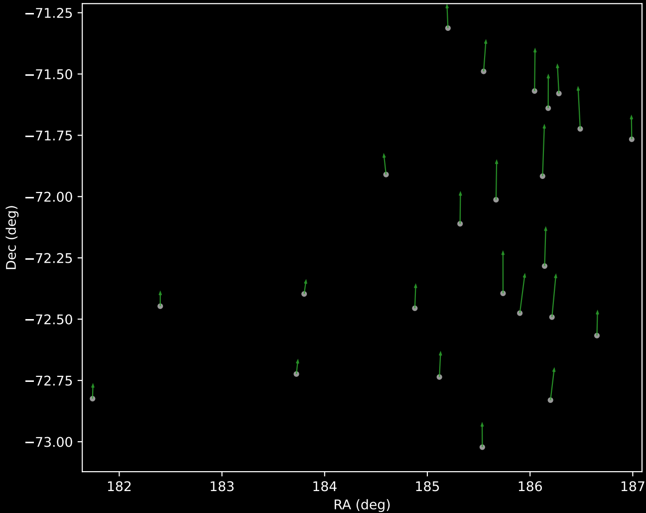
GALAH DR4 Cluster 4 Proper Motion Vectors (n=24)
