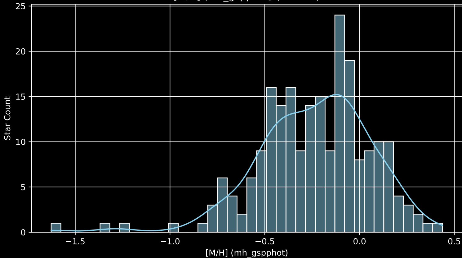
GALAH DR4 Field: [7151] [M/H] (mh_gspphot) (n= 219)
