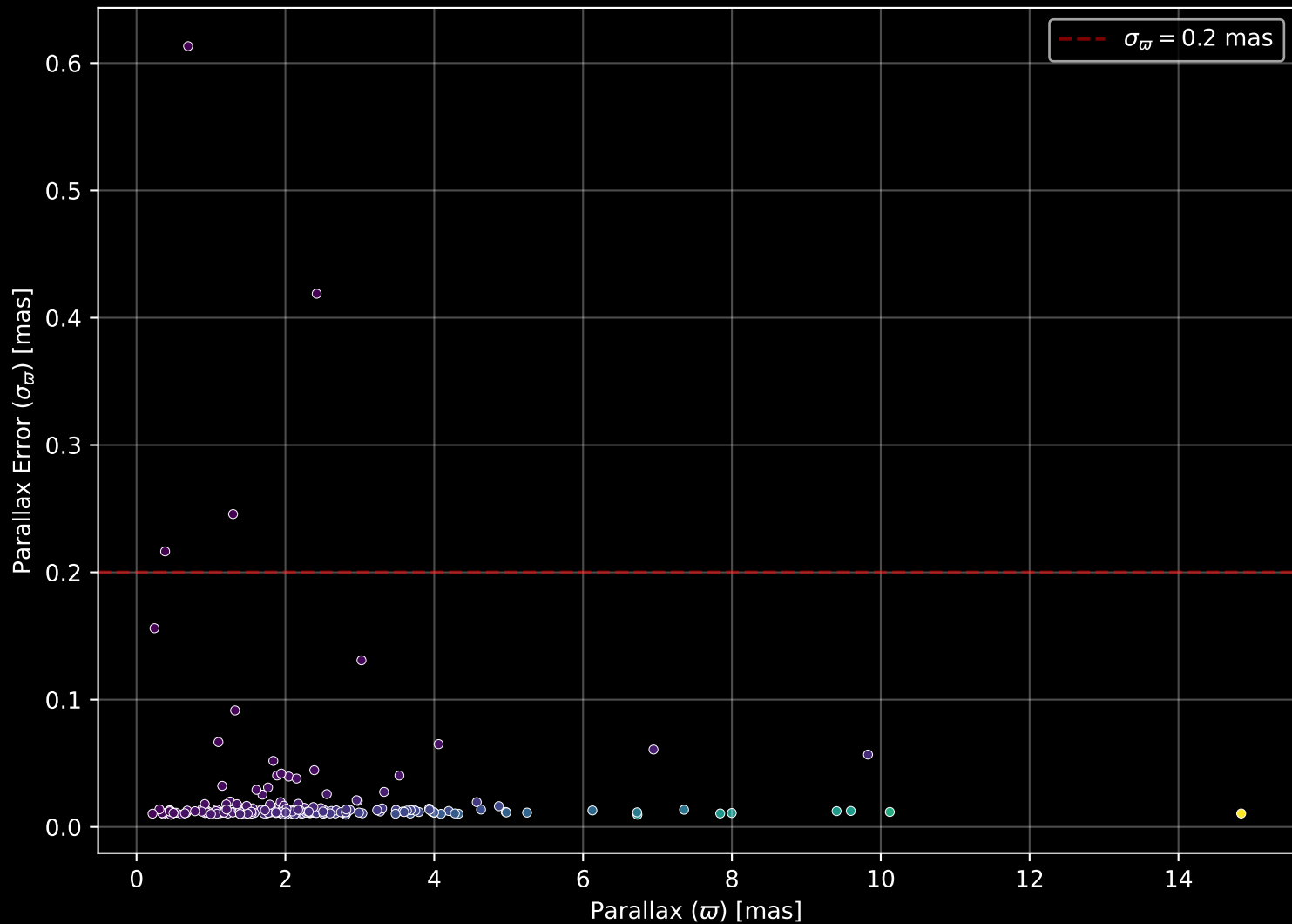
GALAH DR4 Field: [7151] Parallax Quality (n= 220)
