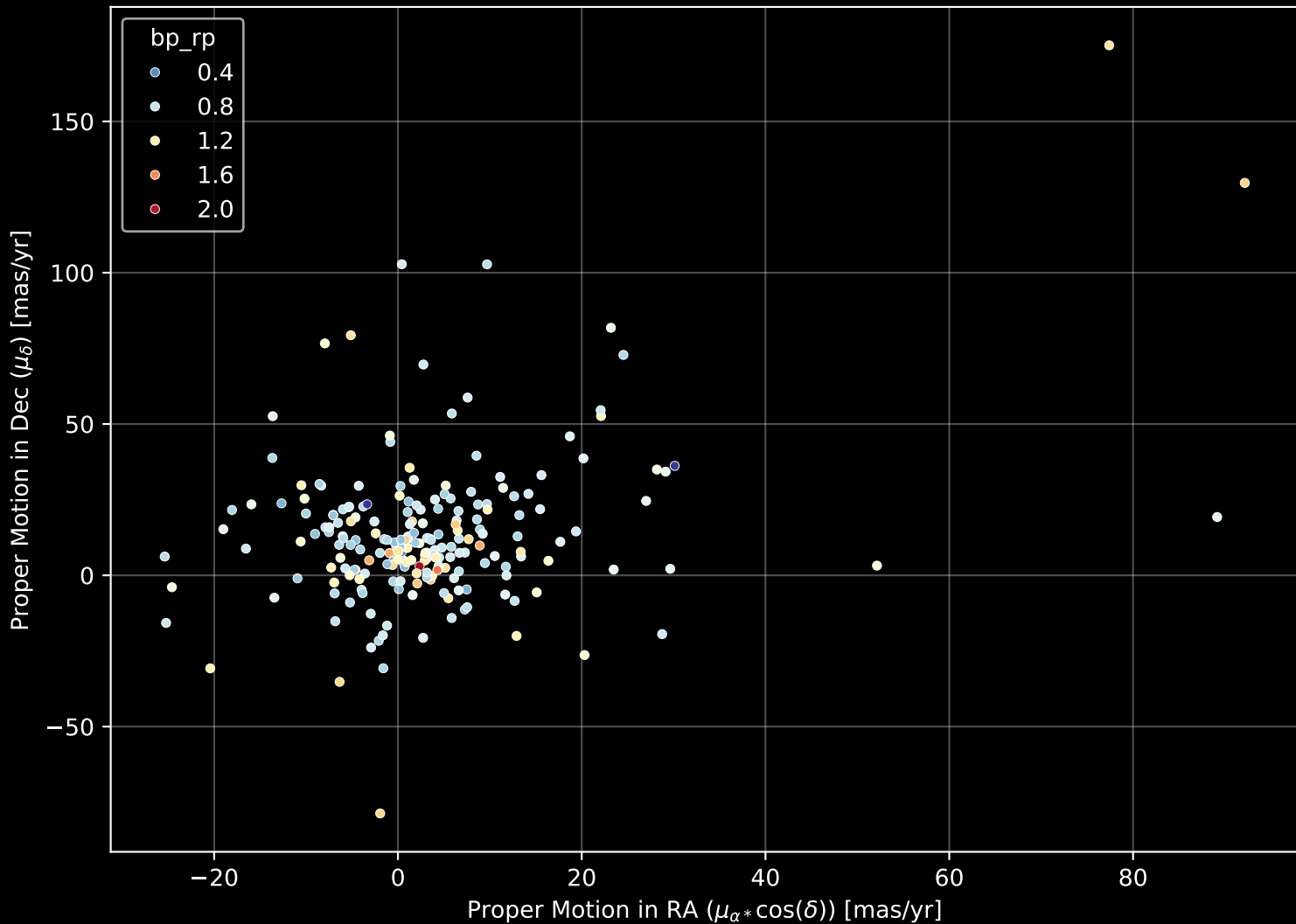
GALAH DR4 Field: [7151] Proper Motion Diagram (n= 220)
